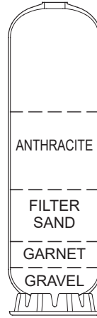
MULTI-MEDIA FILTERS
